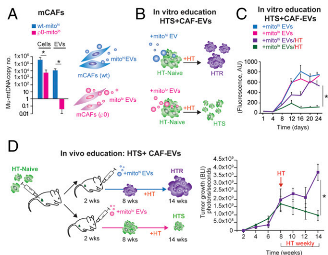
Fig. 4. mCAF-derived EVs educate tumor cells, mediating HTR disease. (A) Mu-mtDNA copy number by qPCR in mCAFs and their EVs; Wt, wild type; ρ0, cells depleted for mtDNA ( Materials and Methods ). The bar graph reports the mean copy number (log 10 scale) of three independent experiments; error bars indicate SD. * P < 0.05 (Student's t test). (B) Schematic showing HTS cells (green) treated with 3 \times 10^9 mCAF-derived EVs (wild-type mtDNA hi or ρ0-mtDNA lo ) once weekly for 4 wk + HT (fulvestrant, 10 μM/wk), leading to the growth of wild-type mtDNA hi -EV-educated cells. (C) Proliferation (shown by Calcein AM staining) of BT474 (HTS cells) cultured for 24 d ± HT (fulvestrant, 10 μM/wk) and treated weekly with 3 \times 10^9 mCAF-derived EVs (wild-type mtDNA hi or ρ0 mtDNA lo ). The mean ± SD for each time point of the growth curve is reported; * P < 0.05 (post hoc t test corrected for multiple comparisons after GLM for repeated measures). (D) Schematic and tumor growth curve of HTS cells (MCF7) injected into the MFP and subsequently educated weekly via retroorbital injection of 3 \times 10^9 with wild-type mito hi or ρ0-mtDNA lo EVs. After 8 wk, HT was administered (fulvestrant, 100 μg/wk) for 6 wk. The mean ± SEM for each time point of the growth curve is reported; * P < 0.05 (post hoc t test corrected for multiple comparisons after GLM for repeated measures).
