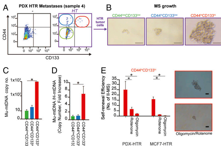
Fig. 6. mtDNA horizontal transfer in vivo preferentially occurs in CSCs, leading to increased self-renewal with hormonal therapy. (A) Representative CD133/CD44 expression by flow analysis of HRT PDX cancer cells and controls (no HT). Briefly, cancer cells were isolated from patient-derived bone metastases (sample 4), grown in culture dishes for 2 wk, and then injected into the MFP of NOD/SCID mice treated with HT (fulvestrant, 1 mg/wk). After 5 mo, tumor tissues were digested, and cancer cells were cultured in vitro and FACS sorted. (B) Representative images of 3D cell cultures (low-attachment plates at day 7) of the three cell populations derived from A. (Scale bars, 100 \mu m.) (C) The mu-mtDNA level is reported as copy number (qPCR, ND1) in FACS-purified cancer cell populations from A. (D) Bar graph showing mtDNA copy number as fold increase of the ratio of murine versus human mtDNA in cell populations from A. (E) Self-renewal potential as secondary mammosphere formation (II-MS) in the presence of mitochondrial poisons administered every 48 h in CD44 hi CD133 hi CSCs at day 7 of 3D culture (rotenone 100 nM, oligomycin 200 nM). Data in C–E are reported as the mean of three independent experiments; error bars indicate SD; * P < 0.05 (student's t test).
