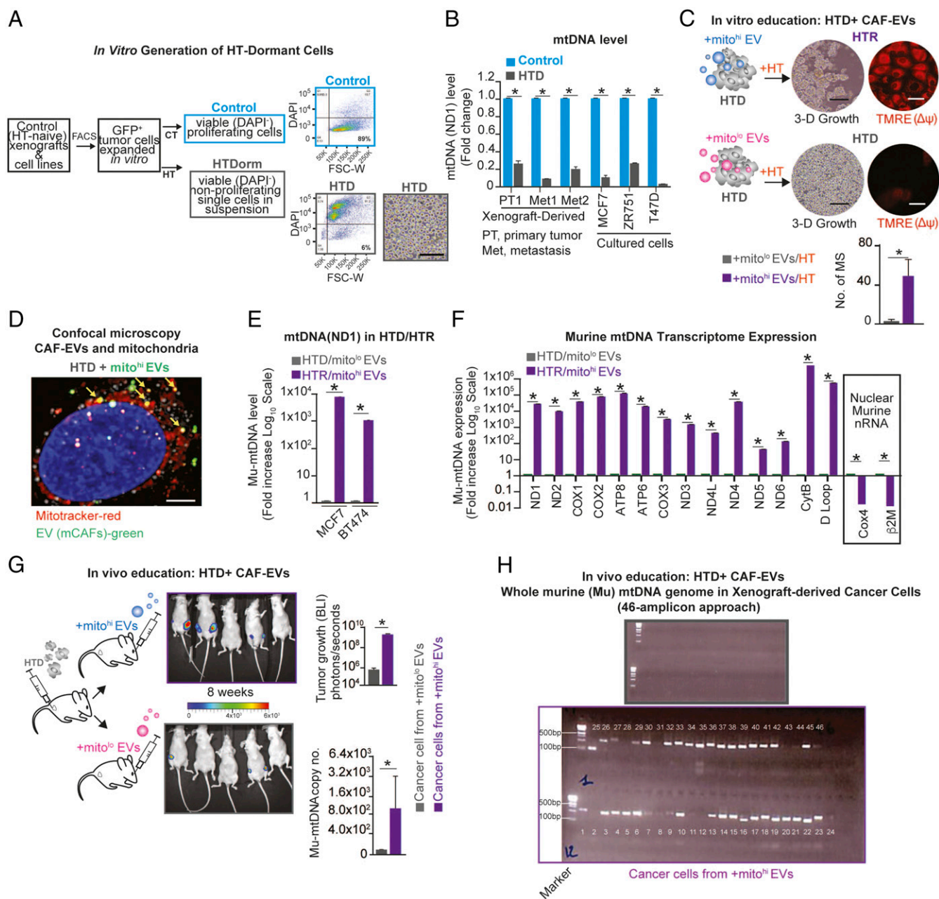
Fig. 5. mCAF-derived EVs promote the exit from HT-induced tumor dormancy. (A) Schematic of the experimental design and representative flow plots: HT-naive cells were FACS isolated from xenografts (GFP + ) or luminal breast cancer cell lines and were treated with HT (fulvestrant, 10 μM/wk) for 2 mo; HTD cancer cells (6% of the viable population, HTDorm) were FACS purified (Dapi - ) and displayed a single-cell (nonproliferating) morphology in 3D. (Scale bar, 100 μm.) (B) mtDNA levels (determined by qPCR and expressed as fold change; naive cells were used as reference) in luminal breast cancer cells and xenograft-derived cells (multiple models) ± HT (fulvestrant, 10 μM) for 2 mo. (C) Dormant MCF7 cells (HTD) were isolated (SI Appendix, Fig. S5) and treated weekly for 4 wk with 3 × 10 9 mCAF-derived EVs (wt-mtDNA hi or ρ0-mtDNA lo ) + HT (fulvestrant, 10 μM/wk). After 40 d, mammosphere (MS) number and mitochondrial membrane potential (Δψ) were determined by TMRE staining (red) in HTR/mito hi -EV- and HTD/mito lo -EV-educated cells. (Scale bars, 15 μm.) (D) Confocal microscopy of HTD cells incubated for 48 h with PKH67 Green-labeled mCAF EVs (green), MitoTracker-labeled mitochondria (red), and EVs colocalized with mitochondria (yellow). (Scale bar, 5 μm.) (E) Mu-mtDNA level (qPCR, ND1) shown as the fold increase (log 10 scale) of the reference HTD from the two HTD-HTR models (MCF7 and BT474) described in C. (F) Mu-mtRNA expression of 14 genes (shown as fold change, -log 10 scale) determined by qRT-PCR in HTR and HTS cells in E (reference HTD cells; MCF7); the expression of nuclear-encoded (nonmitochondrial) murine RNA transcripts was also determined (Cox4, β2M). (G) Schematic, representative photographs, and bar graph showing BLI of tumor growth derived from HTD cells (ZR751 GFP + /Luciferase + cells) injected in the MFP of mice (n = 5 per group) that were treated weekly for 8 wk via retroorbital injection with 3 × 10 9 wt-mito hi or ρ0-mito lo mCAF-derived EVs. Data are shown as mean ± SD at the end point (4 mo); *P < 0.05 (student's t test). The mu-mtDNA level is reported as the copy number (qPCR, ND1) in FACS-purified ZR751 EV-educated cells at the end point of the experiment. (H) Representative gel electrophoresis from whole mu-mtDNA PCR amplification using a set of nuclear mitochondrial sequences (NumtS) excluding overlapping primers in cancer cells from G (grey, mito low EV-derived tumor cells; purple mito hi EV-derived tumor cells) (Materials and Methods). Data in B, C, and E-G are reported as the mean of three independent experiments; error bars indicate SD; In B, C, E, and F, *P < 0.05 (student's t test).
